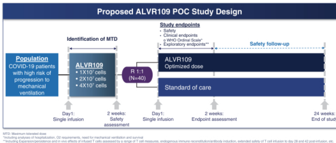
Figure 19. Proposed ALVR109 proof-of-concept trial design
